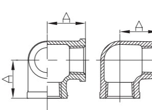
Side Outlet Elbow
