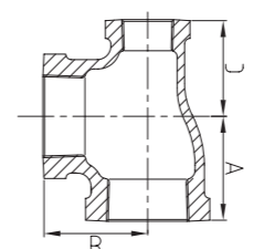
Reducing Tee
