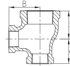
Reducing Tee
