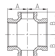
Reducing Cross
